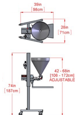
Compact SV Powerlift
